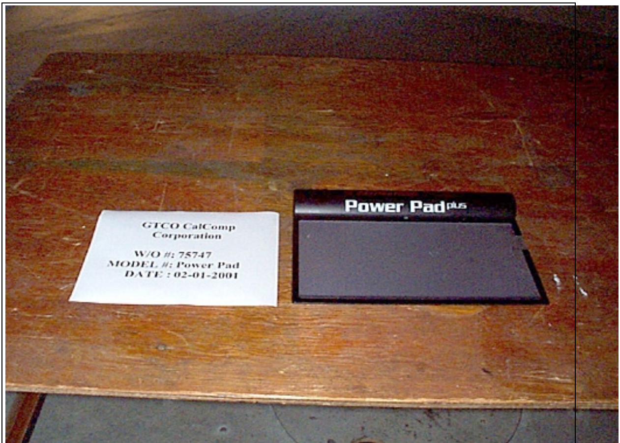
Radiated Emissions - Front View, Face Up Orthogonal
