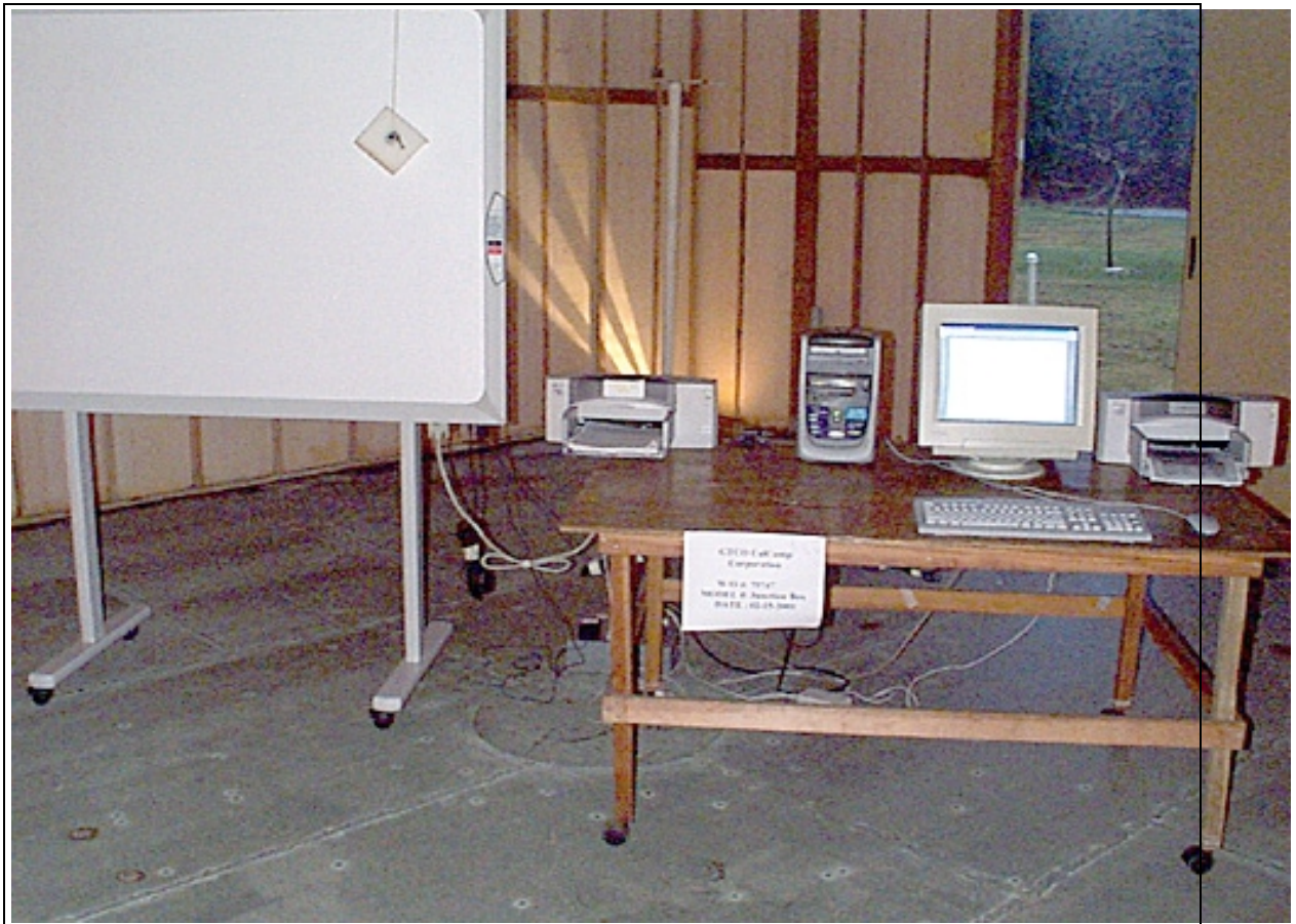
Receiver Radiated Emissions - Front View
