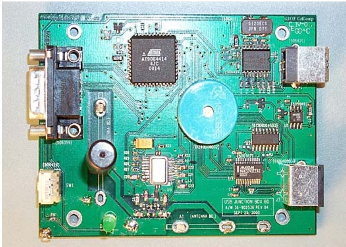
Component side
