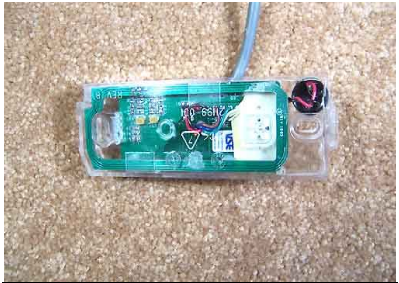
Un-Potted Front
