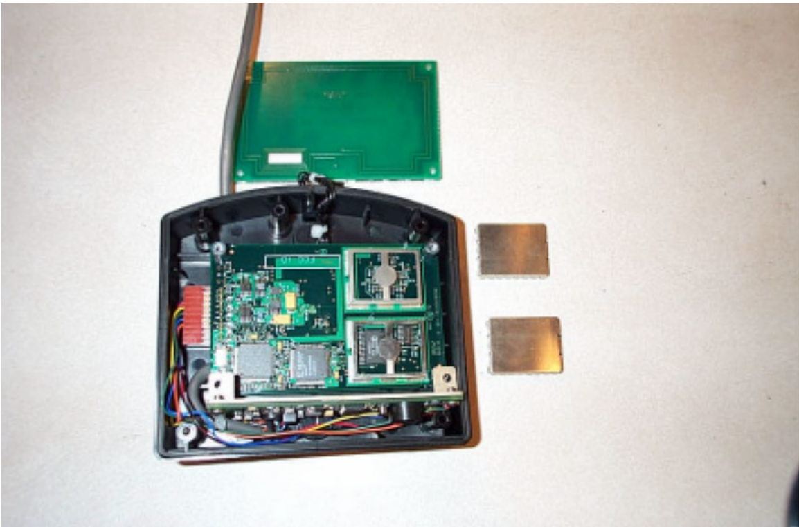
Figure 9.0-3 Top view of Serial CAD Board w/shields removed
