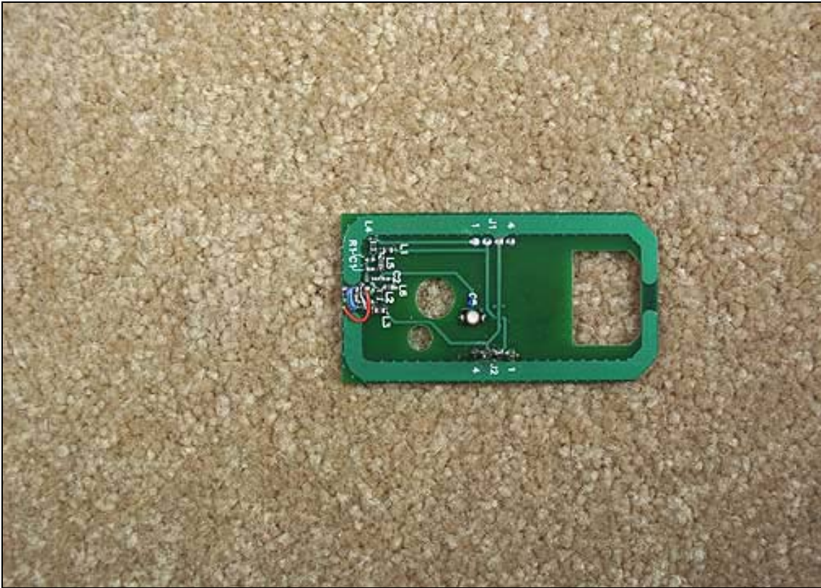
Antenna PCB Component Side
