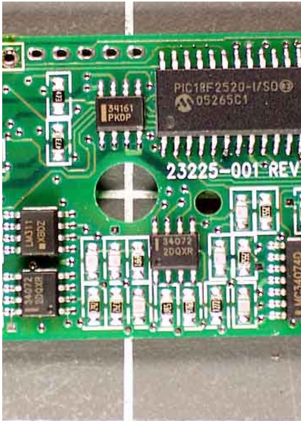
TX PCB Top Closeup 2
