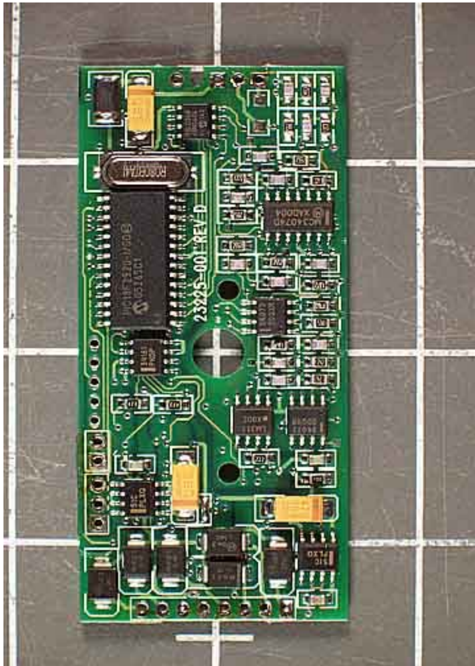
TX PCB Top with Shield Removed
