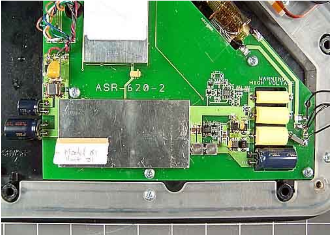
Internal Overview Main PCB Top 1
