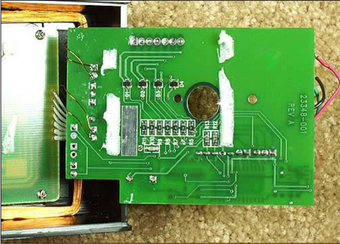
PCB 2 Front
