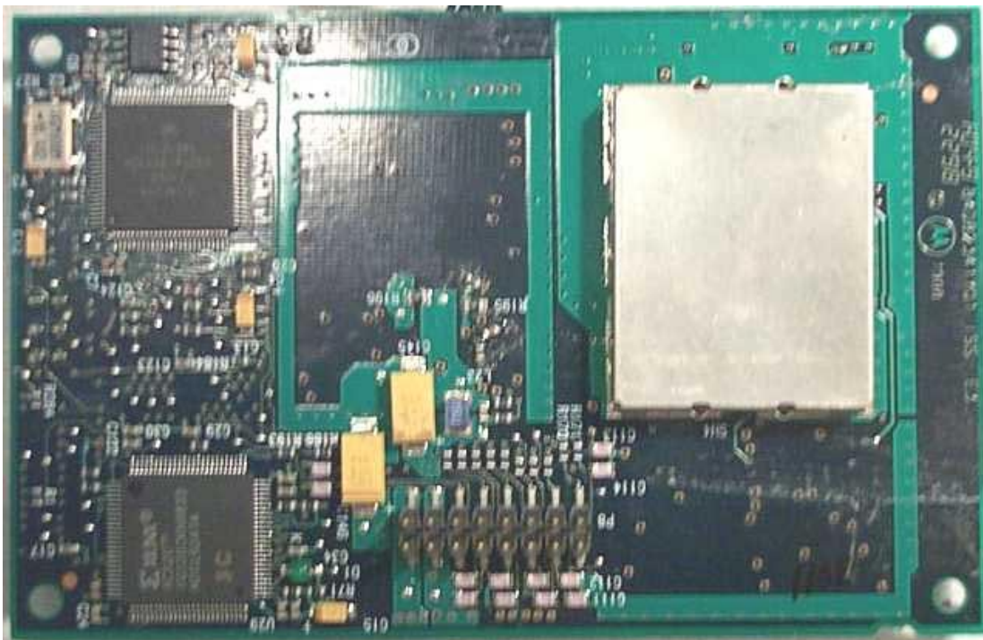
Figure 9.0-3 Transceiver PCB back view
