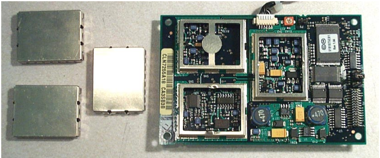
Figure 9.0-2 Transceiver PCB top view with RF shields removed
