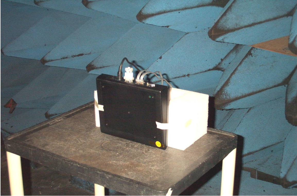
Figure D – 3 Radiated Spurious Emissions Prescan Test Setup, Chamber
