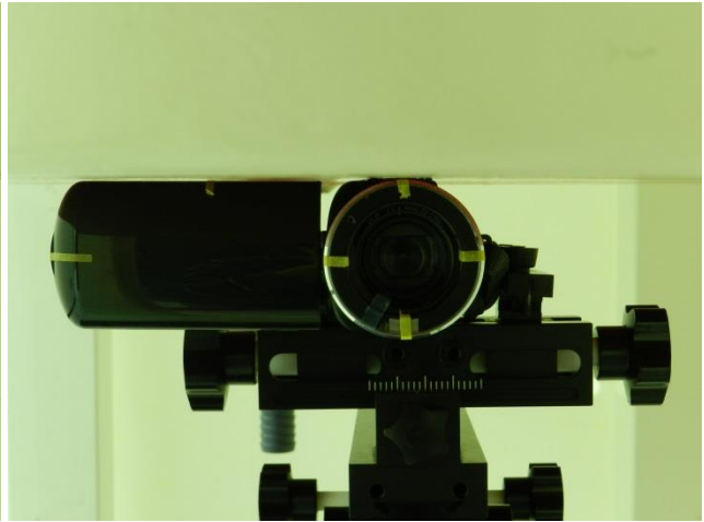
Back of the DUT with Phantom 0 cm Gap (Display screen open)
