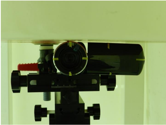
Front of the DUT with Phantom 0 cm Gap (Display screen open)
