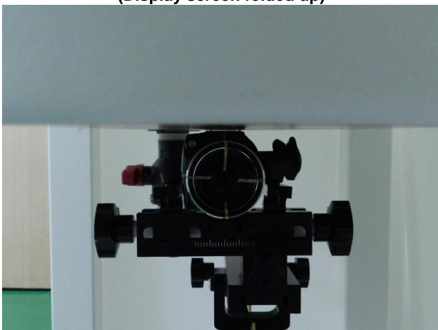
Back of the DUT with Phantom 0 cm Gap (Display screen folded up)
