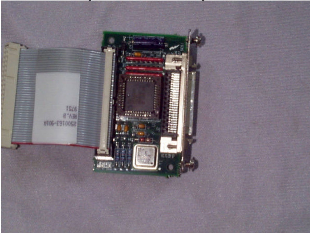
Optional SCSI Interface - Top View
