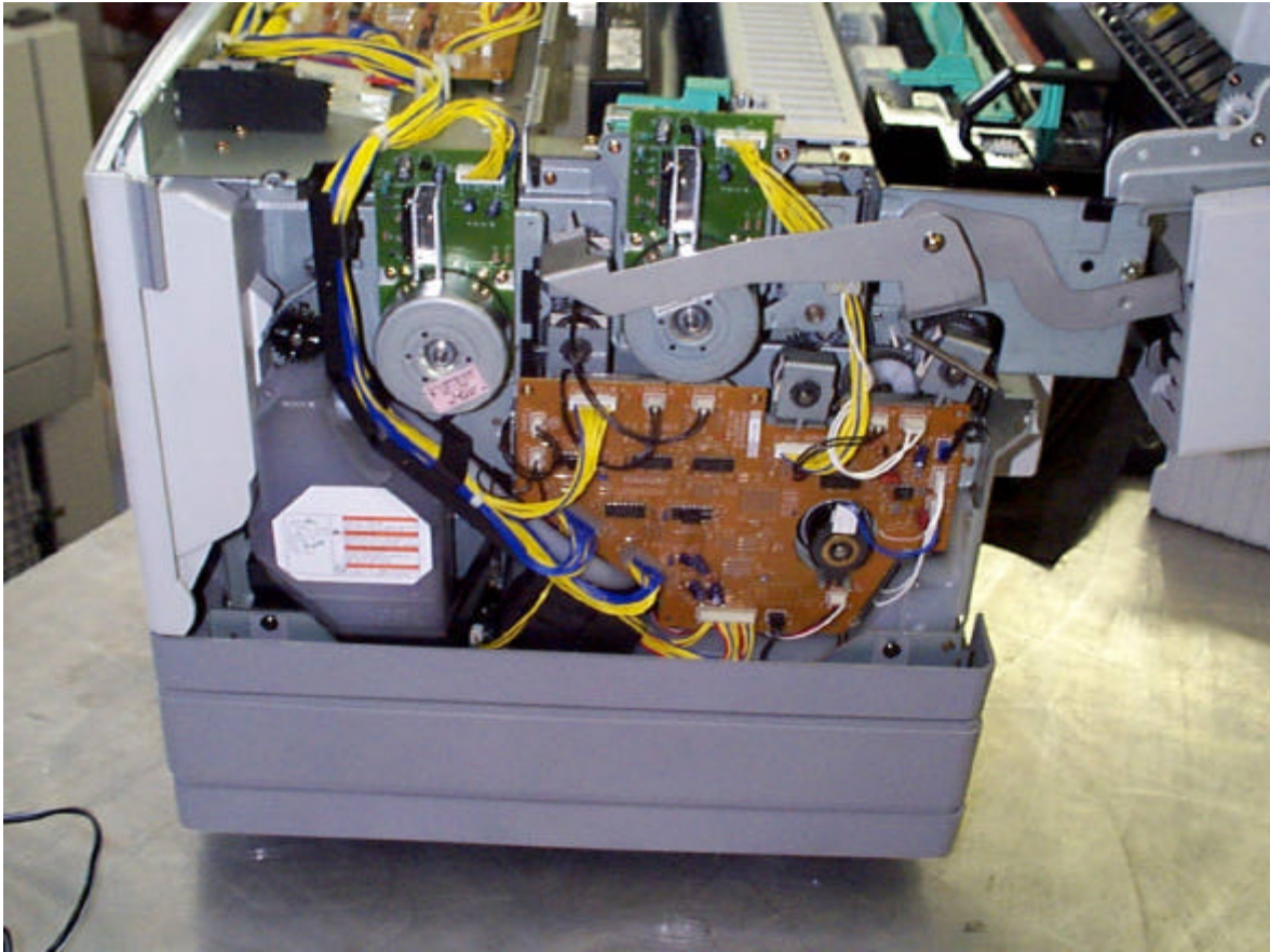
IOD2 Control Board
