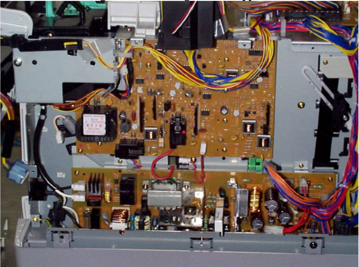
High and Low Voltage Power Supplies
