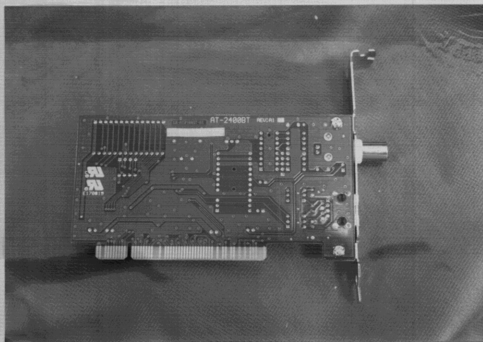
< EUT SOLDERING SIDE VIEW >
