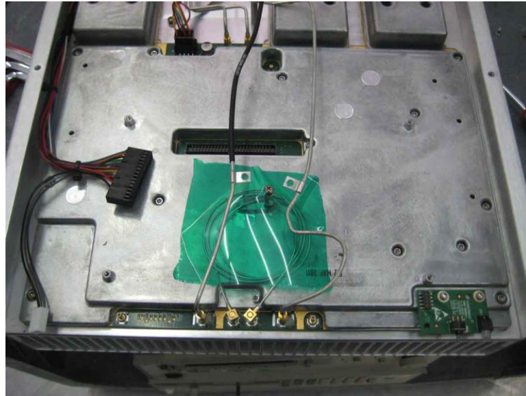
Internal
