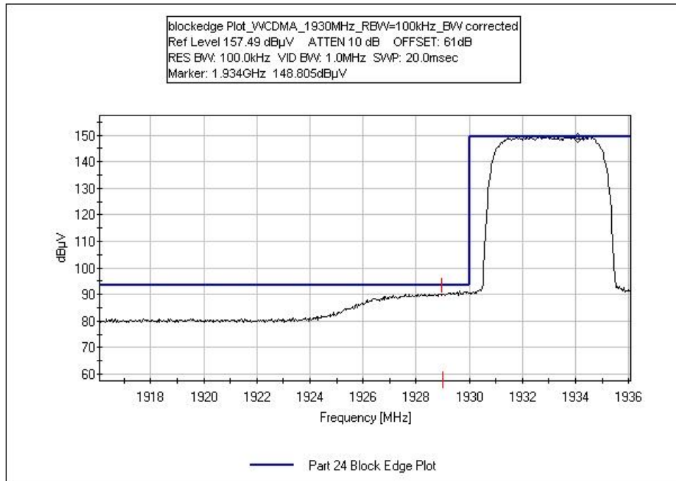
WCDMA – 1930 MHz @ 100 kHz BW Corrected
