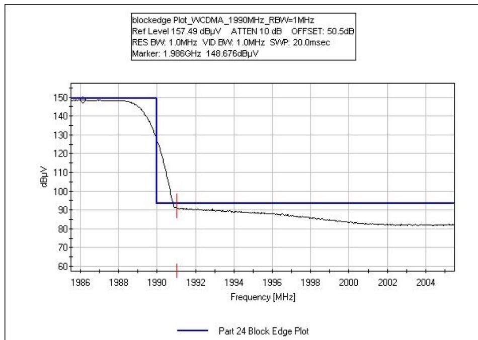
WCDMA – 1990 MHz @ 1MHz
