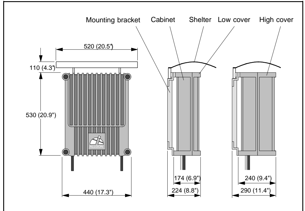
Figure 2-1. Repeater dimensions
