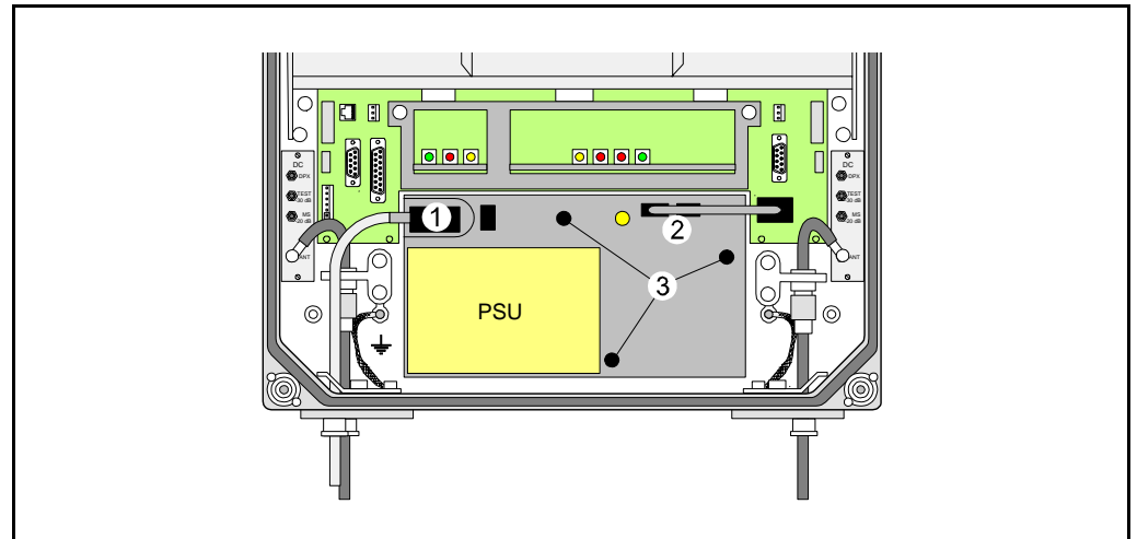
Figure 2-15. Replacing mains PSU with 24V or 48V
