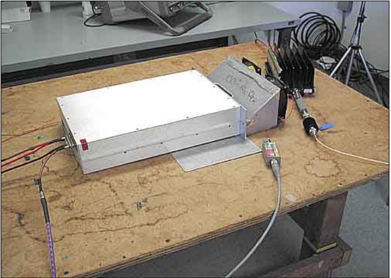
PHOTOGRAPH SHOWING RF POWER OUTPUT TEST SETUP
