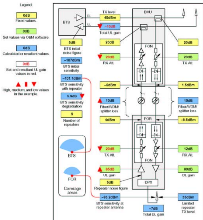
Figure 6-11. Nine FORs, high optical loss, low total uplink gain
