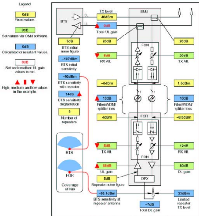
Figure 6-9. Nine FORs, high optical loss, high total uplink gain
