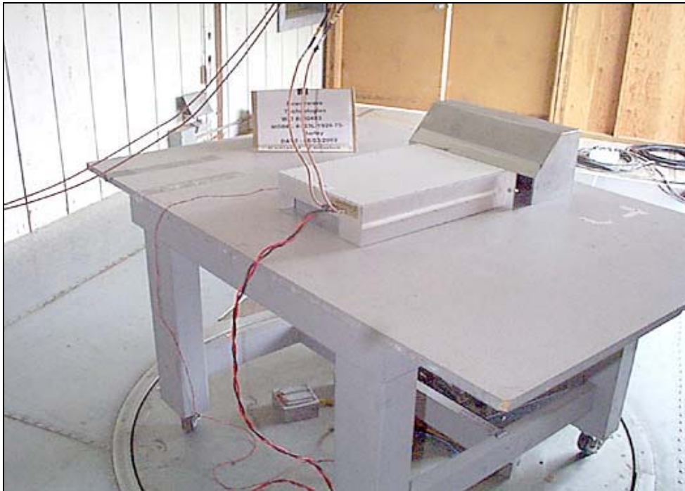
Radiated Emissions - Back View (30-1000 MHz)
