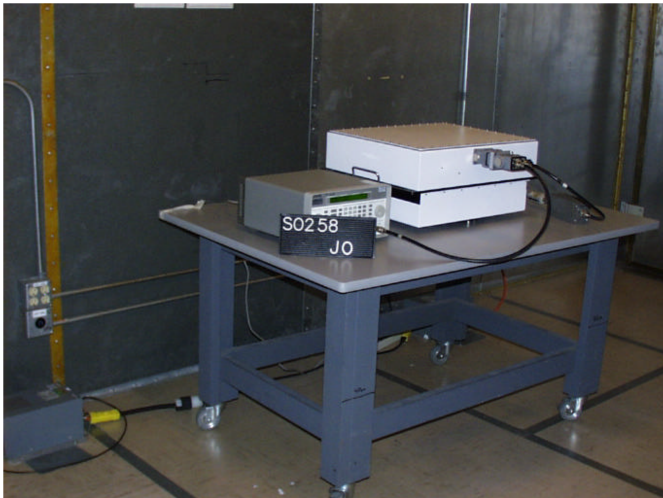
Photograph of Test Setup: Conducted Emissions 10/150/450 kHz - 30 MHz
