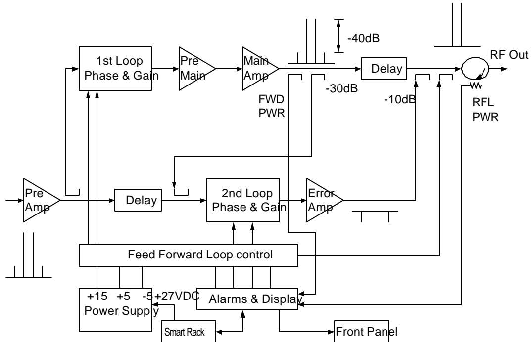
Figure 1-2 Multi-Carrier Power Amplifier Functional Block Diagram
