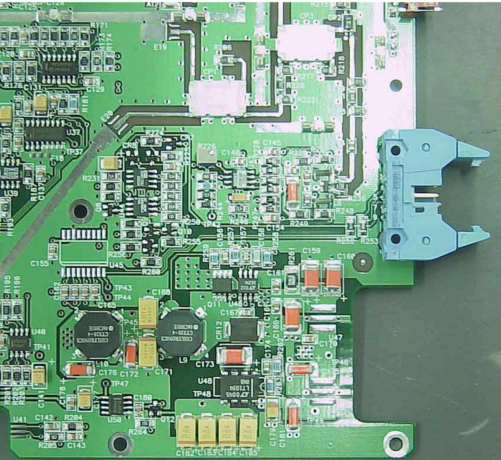
MULTIFUNCTION BOARD FRONT B
