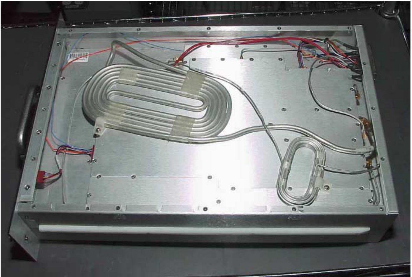
TOP VIEW WITHOUT TOP COVER
