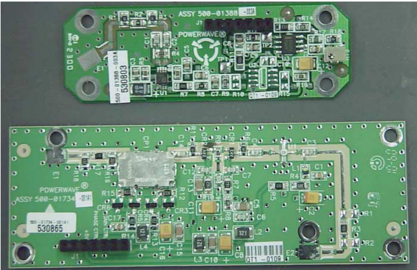
1 ST LOOP & PREAMP FRONT
