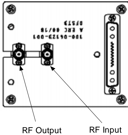
Figure 2-3. Amplifier RF Connector
