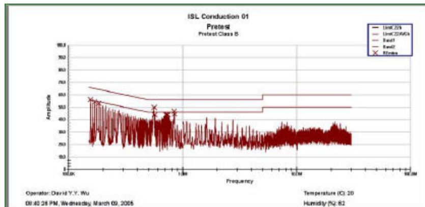
Graph 2.2.1 Power Line Conducted Emissions (Hot)
