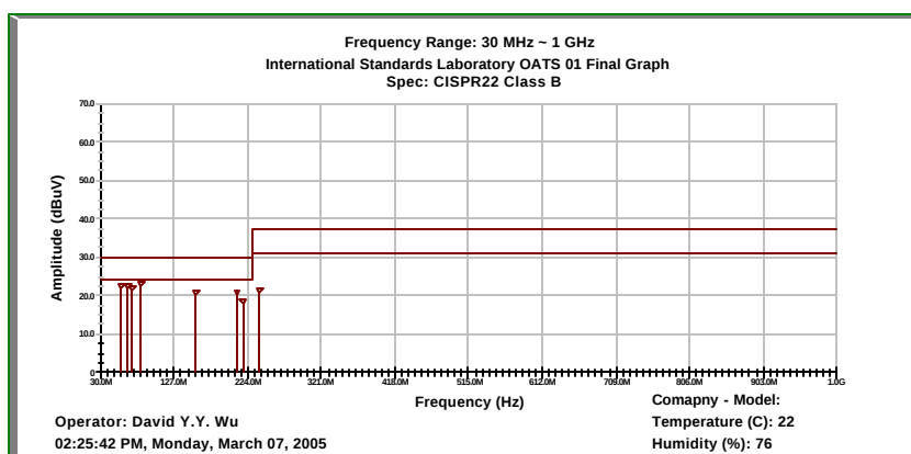
Graph 3.2.2 Open Field Radiated Emissions (Vertical)
