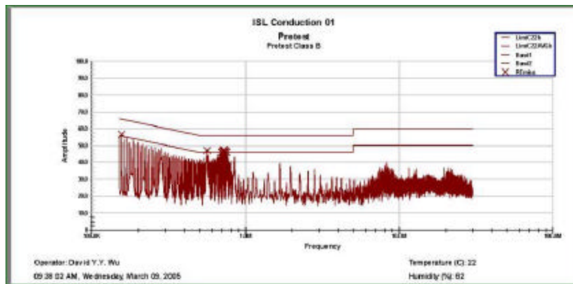
Graph 2.3.2 Power Line Conducted Emissions (Neutral)
