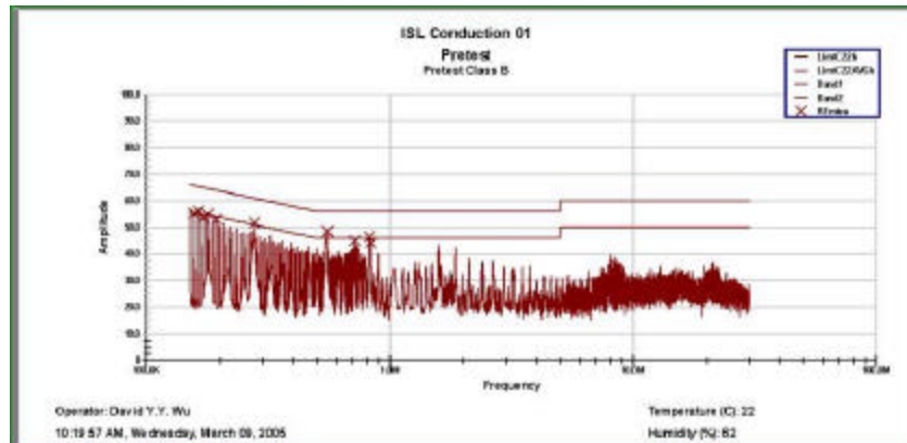
Graph 2.3.1 Power Line Conducted Emissions (Hot)
