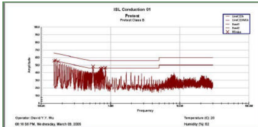
Graph 2.2.2 Power Line Conducted Emissions (Neutral)
