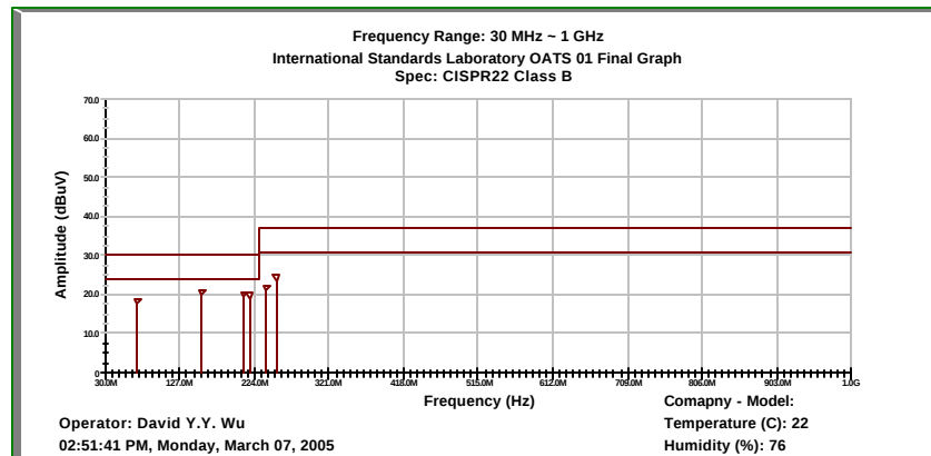
Graph 3.2.1 Open Field Radiated Emissions (Horizontal)
