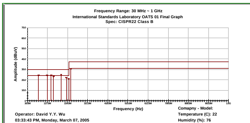
Graph 3.3.1 Open Field Radiated Emissions (Horizontal)
