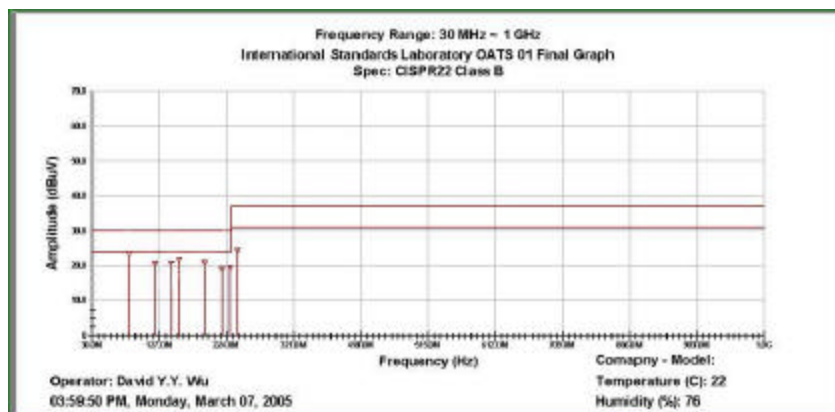
Graph 3.3.2 Open Field Radiated Emissions (Vertical)
