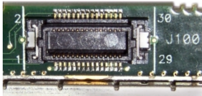
Figure 9. Data Interface Connector (As viewed from above)
