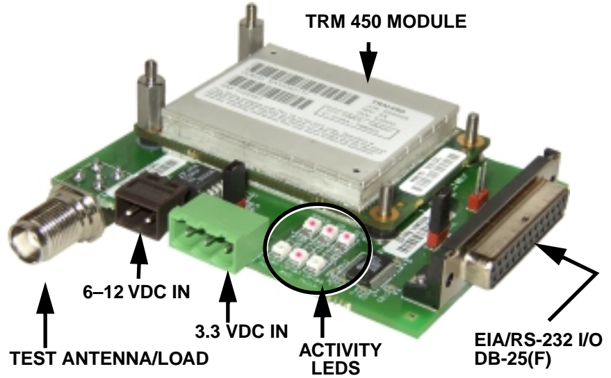
Figure 10. Test and Evaluation PCB Assembly (With TRM 450 module installed and retainers on RF connector end.)
