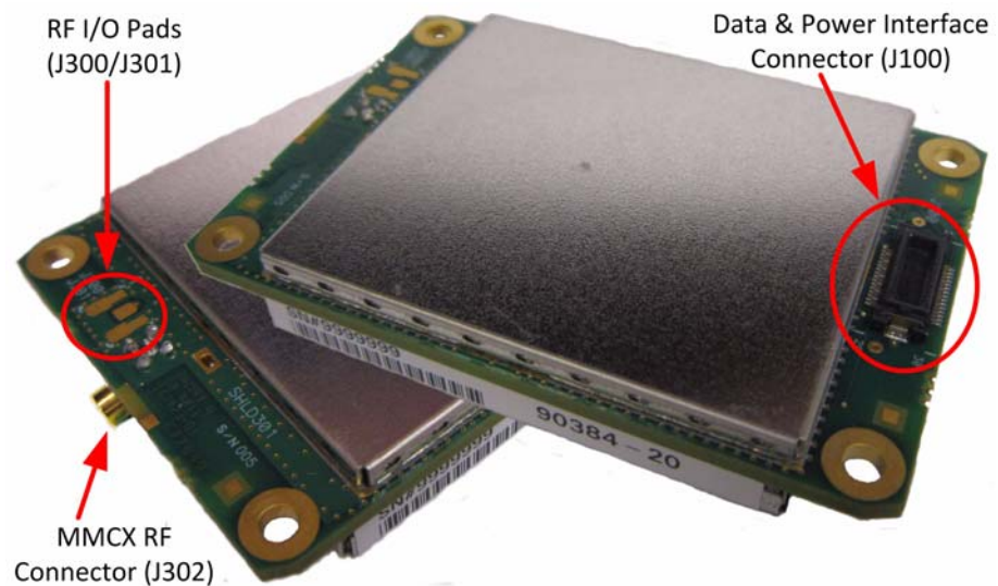
Figure 4. Top and Bottom Views Showing External Connections
