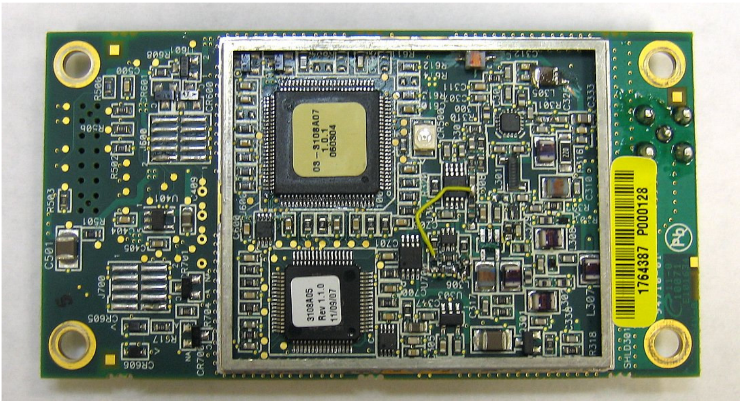
ROR Board – Digital Circuitry Side, shield removed
