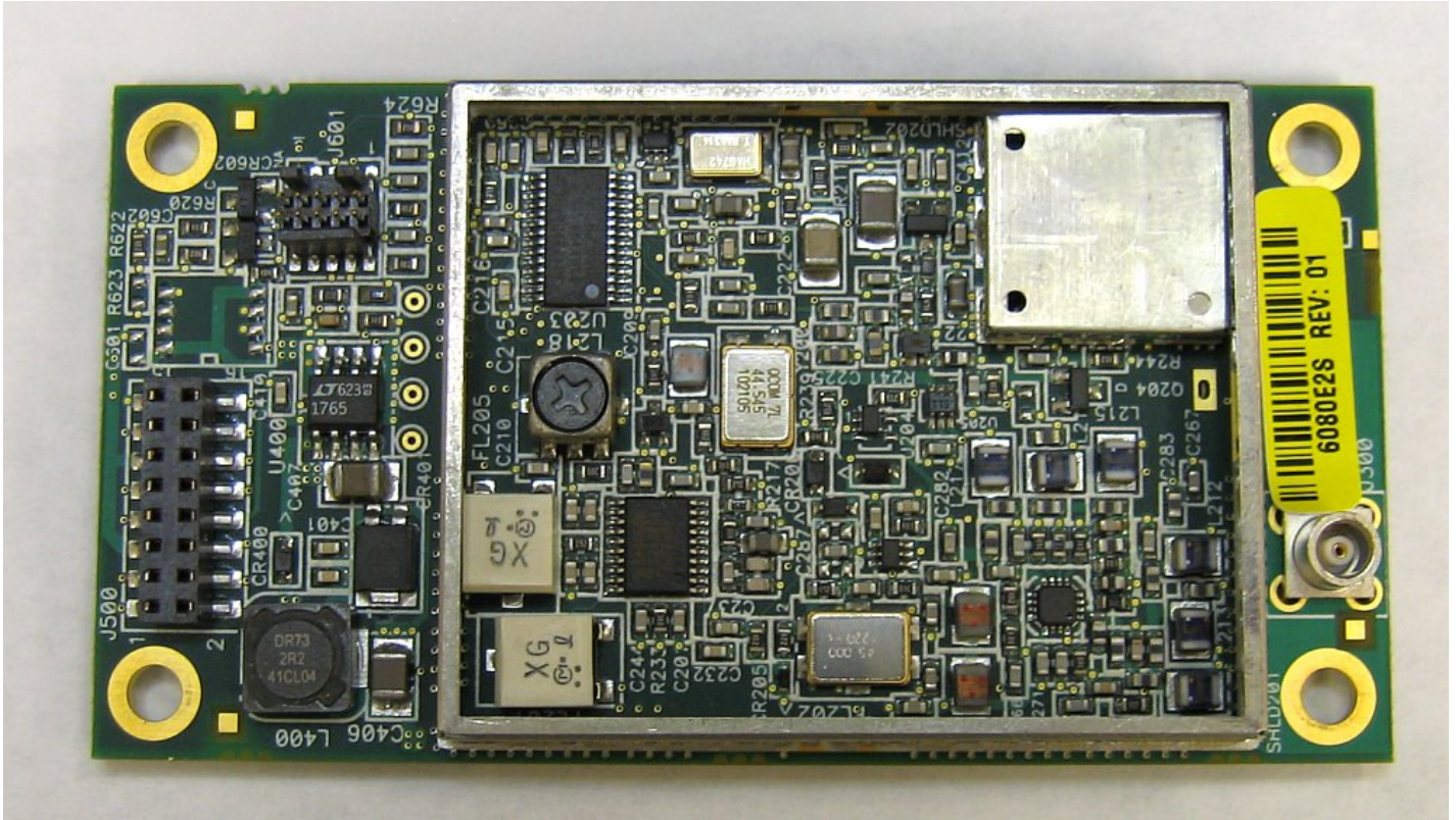
ROR Board – Digital Circuitry Side, shield removed
