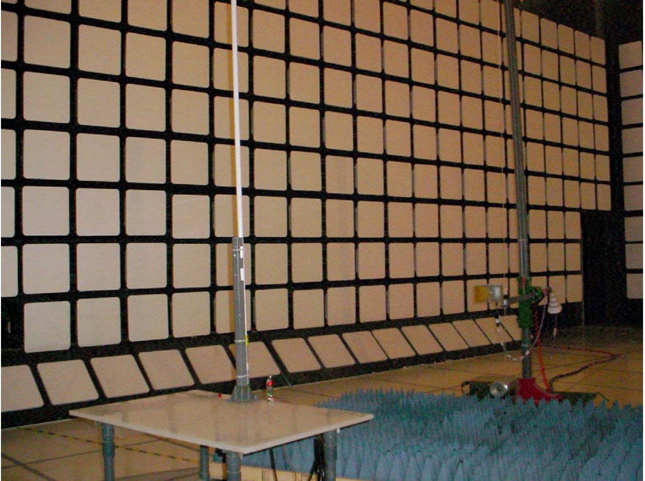
Radiated Emissions @ 3 m EUT with 9.15 dBi Omni Directional Antenna, Orthogonal Position 3
