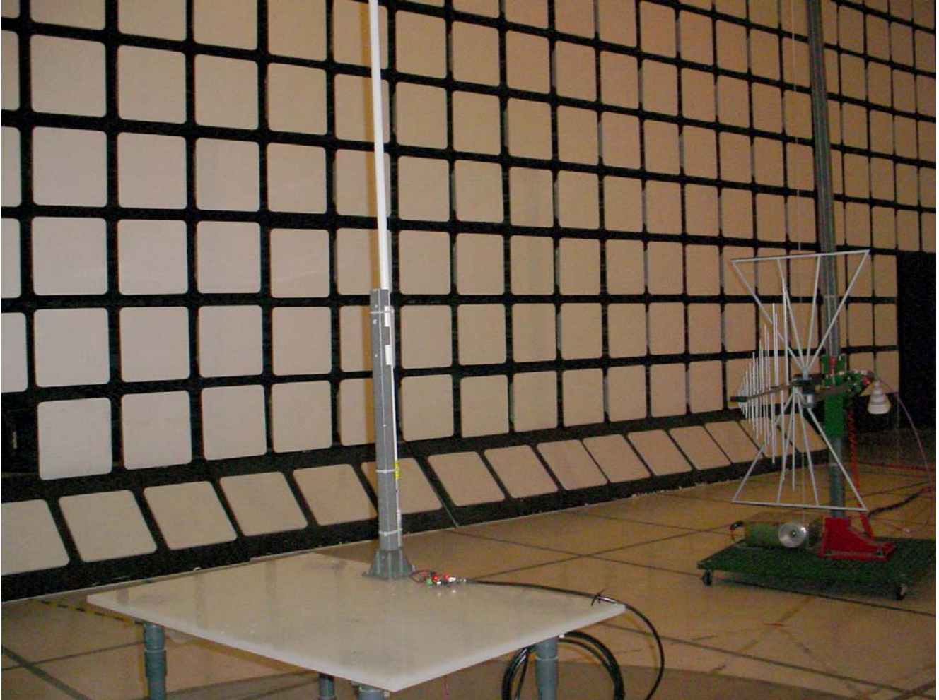
Radiated Emissions @ 3 m EUT with 9.15 dBi Omni Directional Antenna, Orthogonal Position 1
