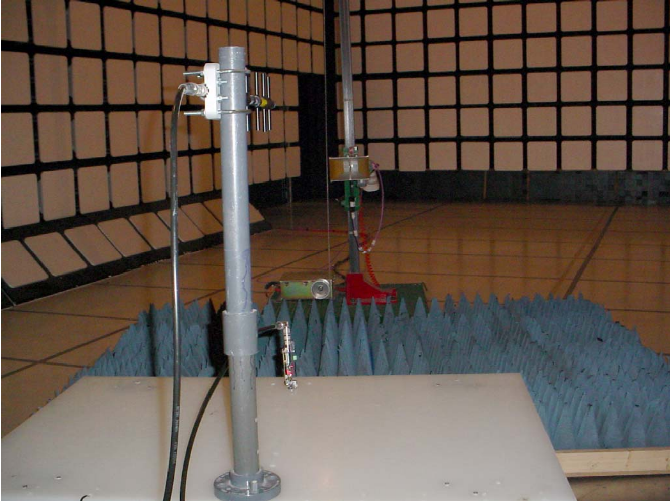
Radiated Emissions @ 3 m EUT with 12.15 dBi Yagi Antenna, Orthogonal Position 3
