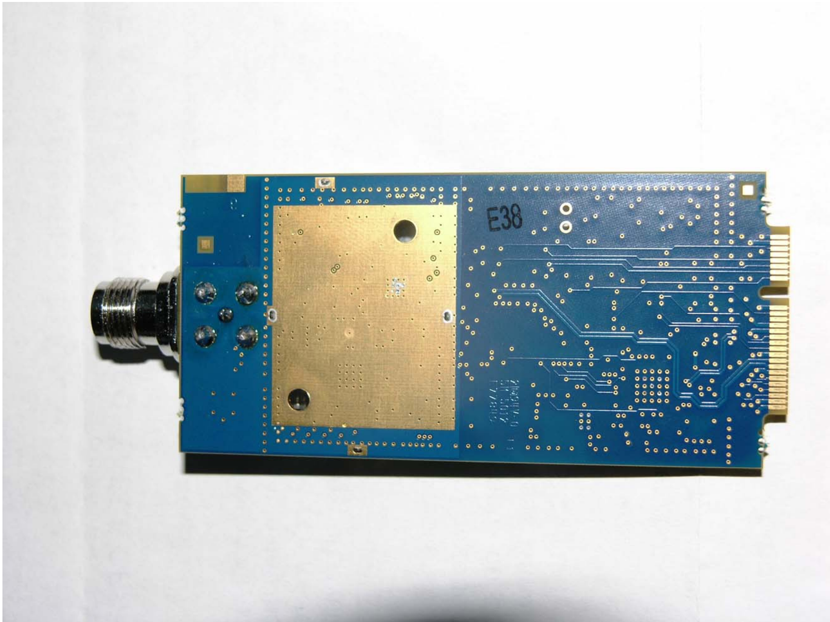
GE MDS LLC. 900MHz OEM DTS / FHSS Module, Model: NX915 FCC ID: E5MDS-NX915, IC: 101D-NX915
