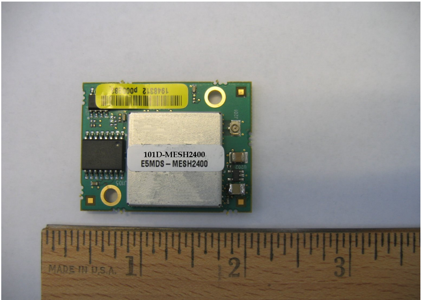
Photographs of original device with shield which is identical to the shield for this application
