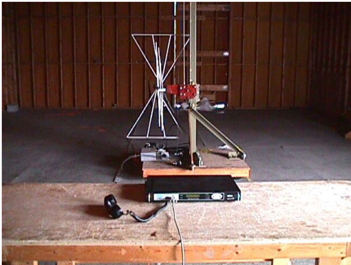
Transmitter Radiated Emissions Test Setup (at 3 meters distance)
