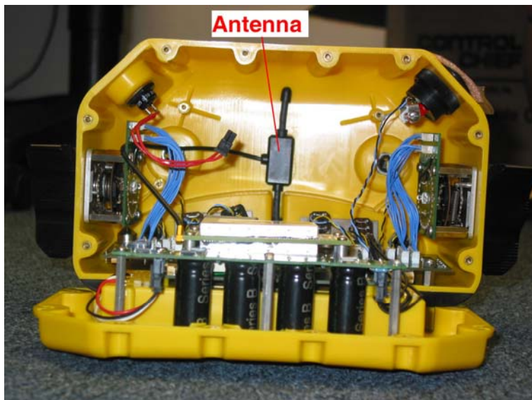
Antenna Location on Inside Front of Device
