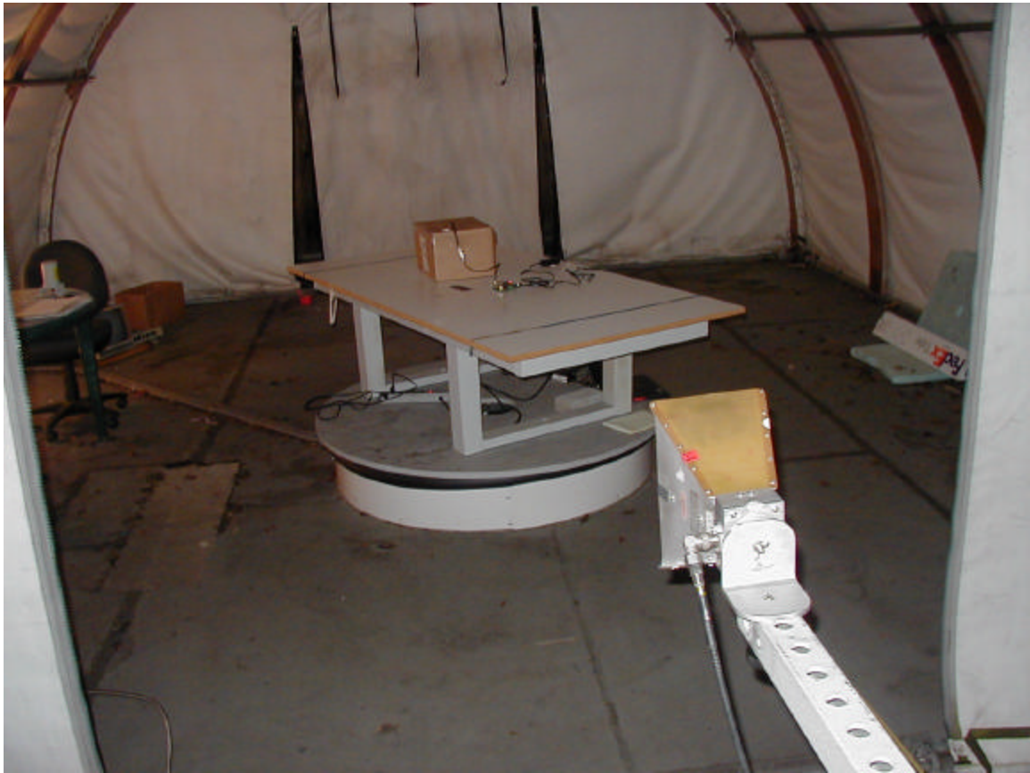
(1/2 Wave Antenna)
