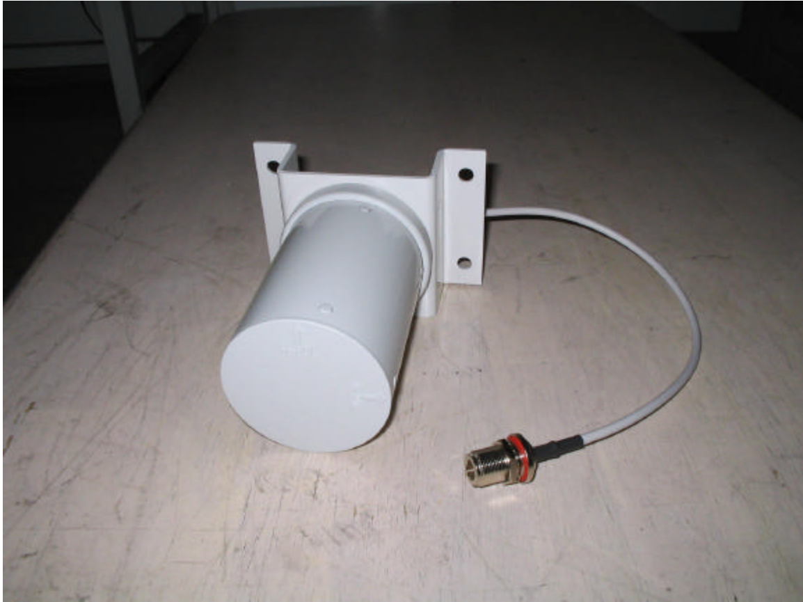
2.4GHz Yagi antenna, Manufacture: MAXRAD (M/N: MYP24010PT) 10dBi gain
