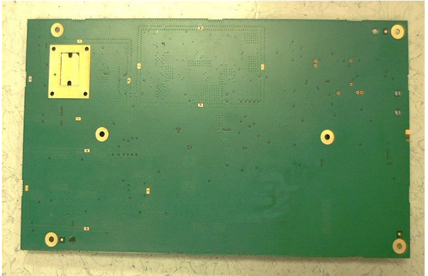
Back side of PCB 2 of 2
