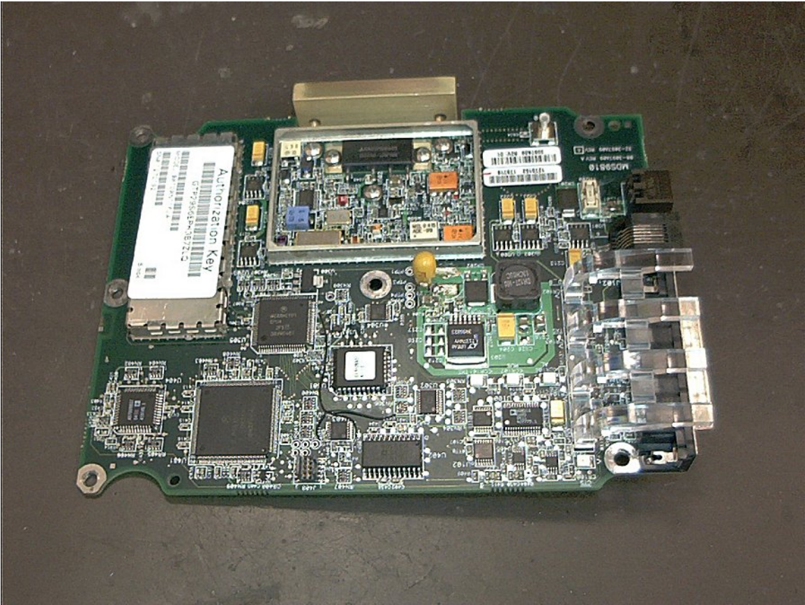
9810 PCB
