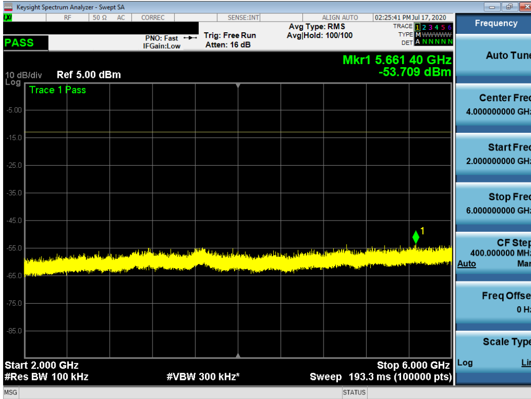
Plot 7-20. Conducted Spurious Plot (QPSK, 6RB, RB Offset 5)
