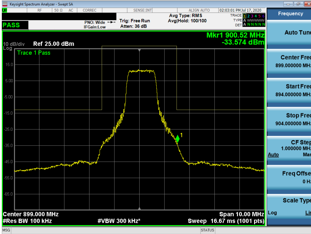
Plot 7-28. Band Edge Plot (QPSK, 6RB, RB Offset 5)
