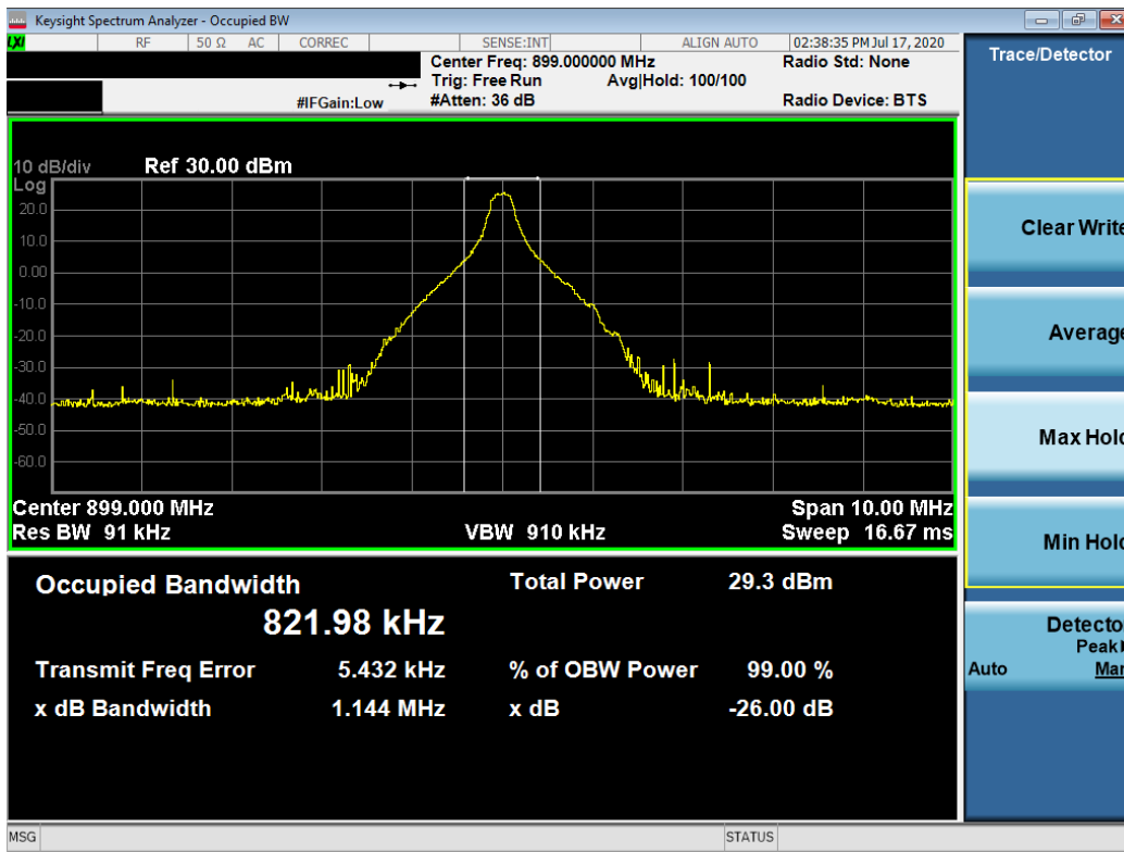
Plot 7-12. Occupied Bandwidth Plot (16-QAM, 1RB, RB Offset 7)
