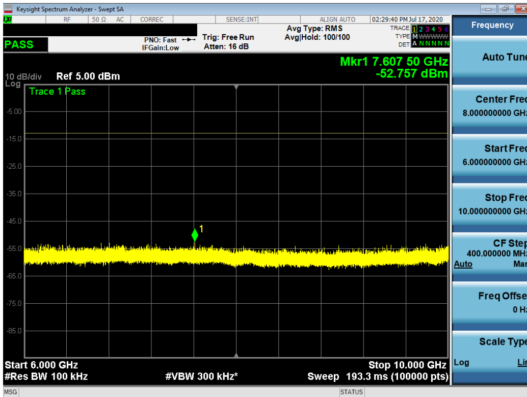
Plot 7-15. Conducted Spurious Plot (QPSK, 1RB, RB Offset 0)
