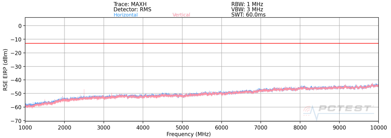
Plot 7-35. Radiated Spurious Plot (LTE Band 8)
