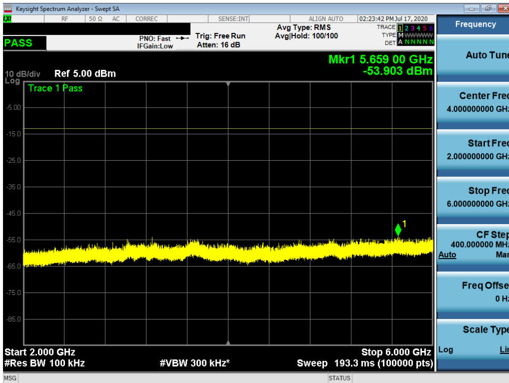
Plot 7-23. Conducted Spurious Plot (QPSK, 15RB (Full), RB Offset 0)
