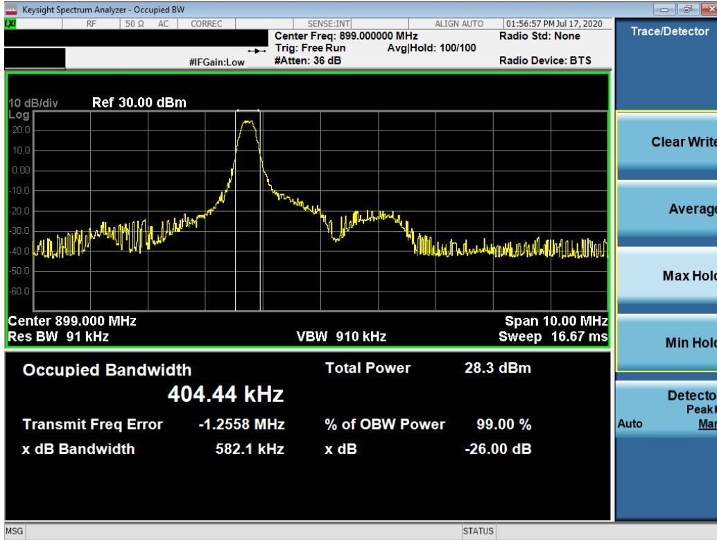
Plot 7-10. Occupied Bandwidth Plot (QPSK, 1RB, RB Offset 7)
