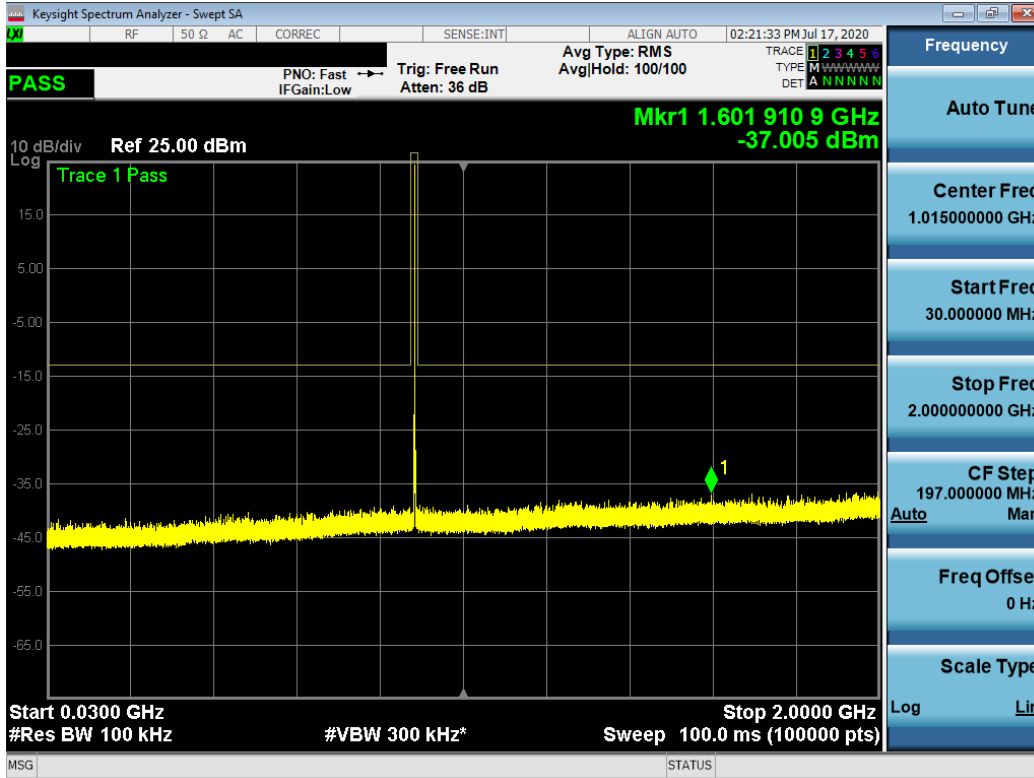
Plot 7-16. Conducted Spurious Plot (QPSK, 1RB, RB Offset 14)
