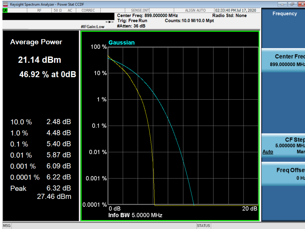
Plot 7-31. Peak to Average Ratio (QPSK, Full RB)
