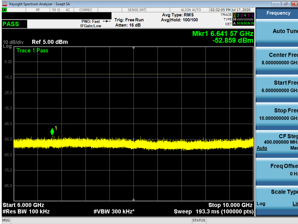
Plot 7-24. Conducted Spurious Plot (QPSK, 15RB (Full), RB Offset 0)
