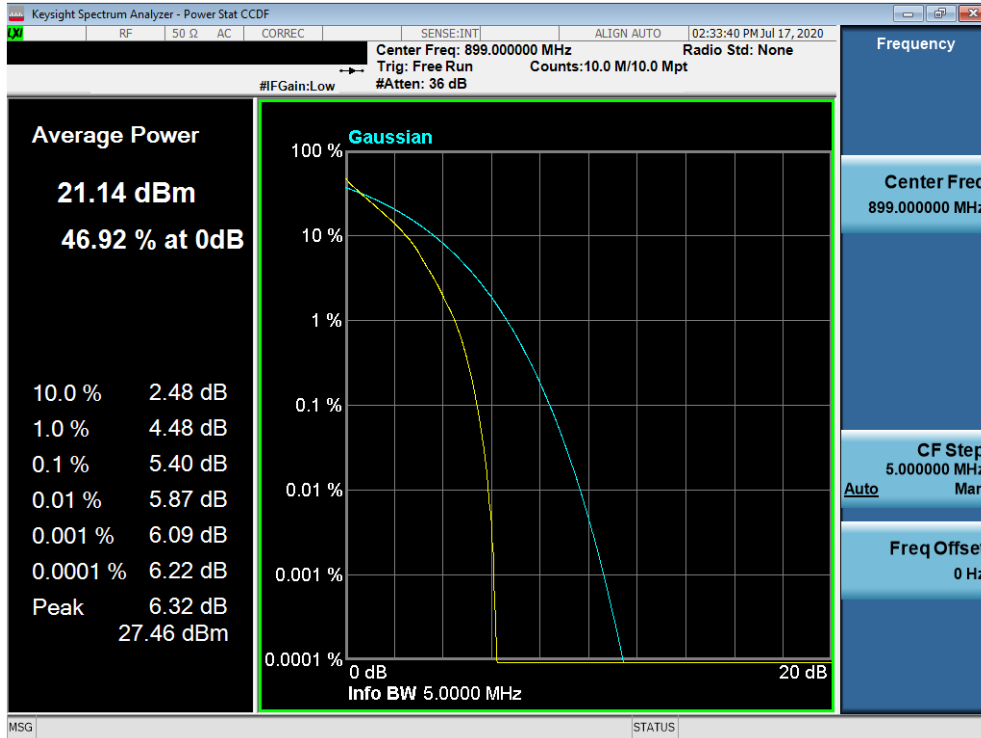
Plot 7-33. Peak to Average Ratio (16-QAM, Full RB)
