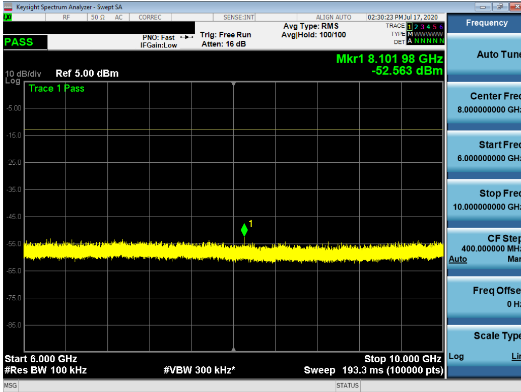
Plot 7-18. Conducted Spurious Plot (QPSK, 1RB, RB Offset 14)
