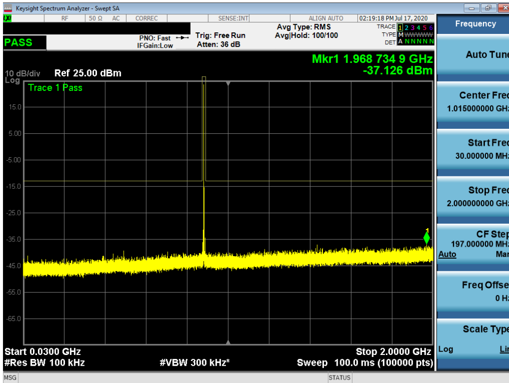
Plot 7-13. Conducted Spurious Plot (QPSK, 1RB, RB Offset 0)
