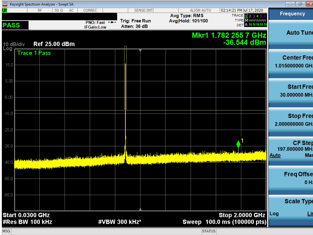
Plot 7-22. Conducted Spurious Plot (QPSK, 15RB (Full), RB Offset 0)
