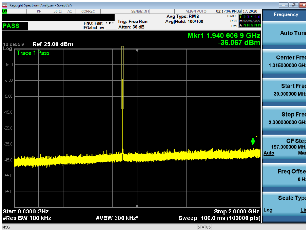
Plot 7-19. Conducted Spurious Plot (QPSK, 6RB, RB Offset 5)
