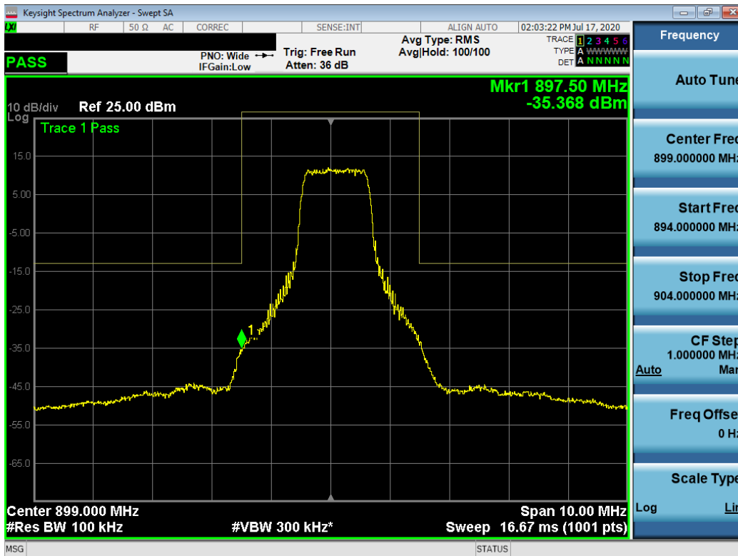
Plot 7-27. Band Edge Plot (QPSK, 6RB, RB Offset 5)
