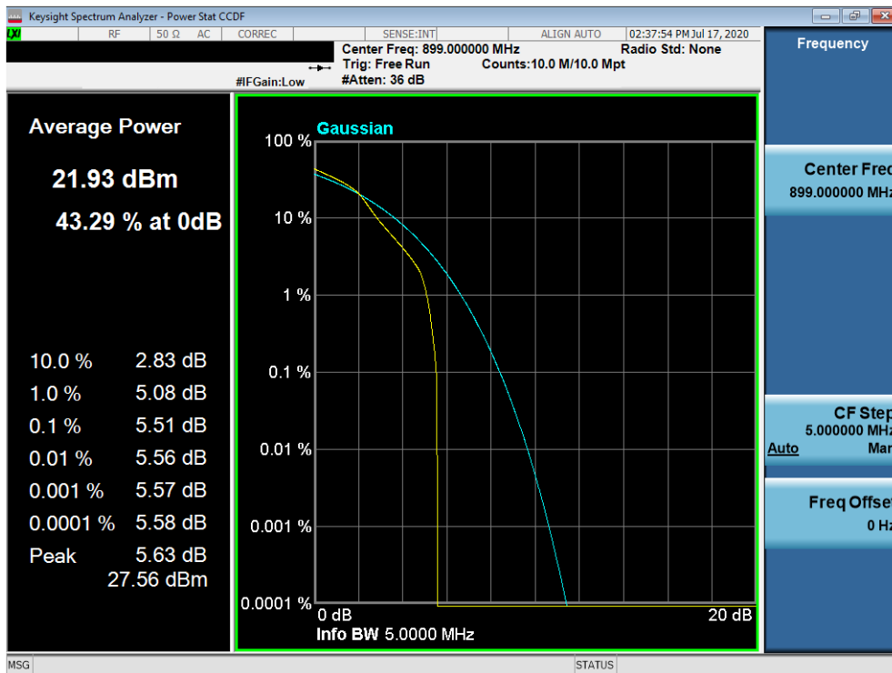
Plot 7-34. Peak to Average Ratio (16-QAM, 1RB Offset 7)
