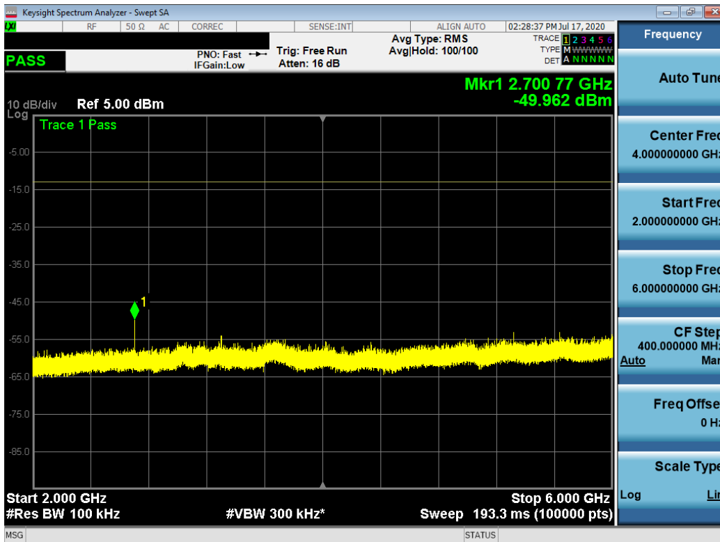
Plot 7-17. Conducted Spurious Plot (QPSK, 1RB, RB Offset 14)
