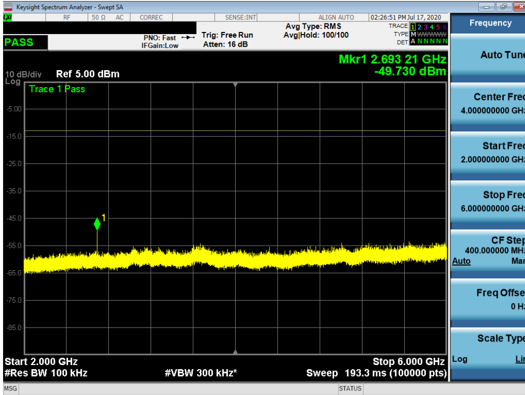
Plot 7-14. Conducted Spurious Plot (QPSK, 1RB, RB Offset 0)
