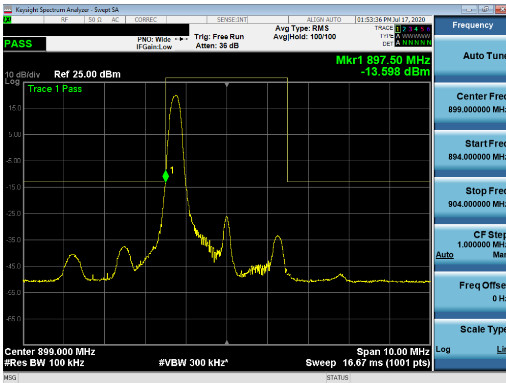
Plot 7-25. Band Edge Plot (QPSK, 1RB, RB Offset 0)
