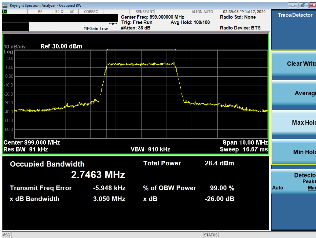
Plot 7-11. Occupied Bandwidth Plot (16-QAM, 15RB (Full), RB Offset 0)
