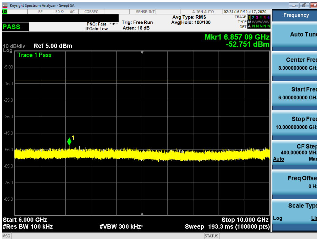
Plot 7-21. Conducted Spurious Plot (QPSK, 6RB, RB Offset 5)
