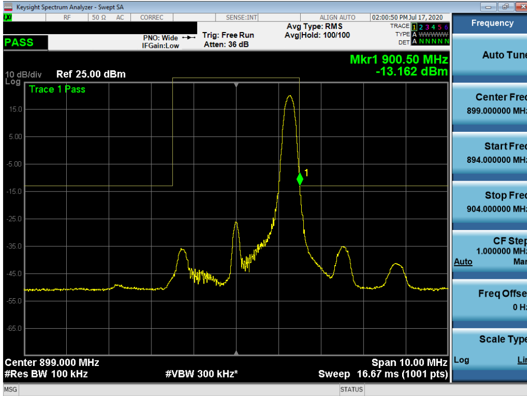
Plot 7-26. Band Edge Plot (QPSK, 1RB, RB Offset 14)
