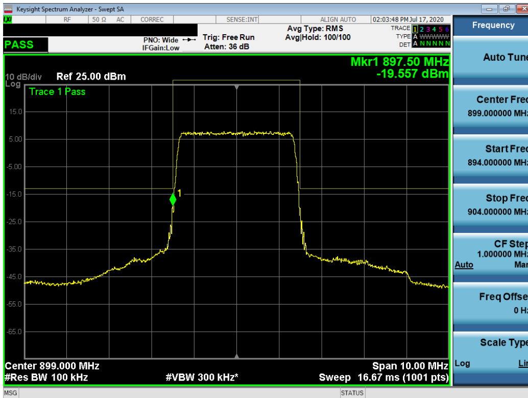
Plot 7-29. Band Edge Plot (QPSK, 15RB (Full), RB Offset 0)
