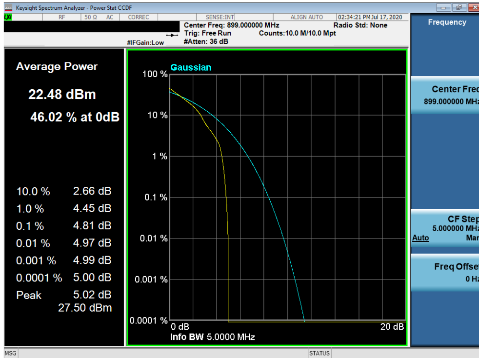
Plot 7-32. Peak to Average Ratio (QPSK, 1RB Offset 7)
