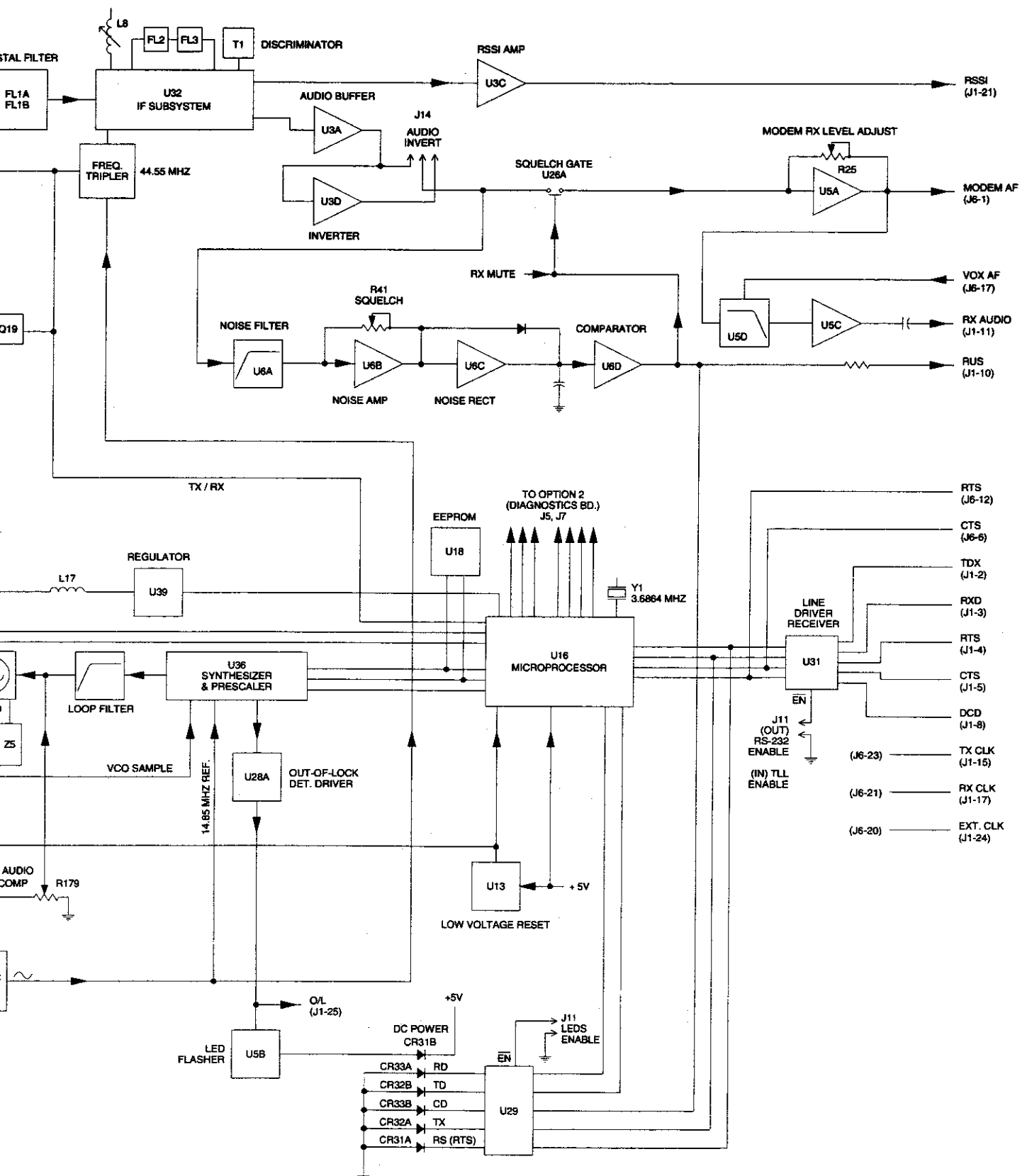
Figure 5-1 MDS 4310 Transceiver Block Diagram
