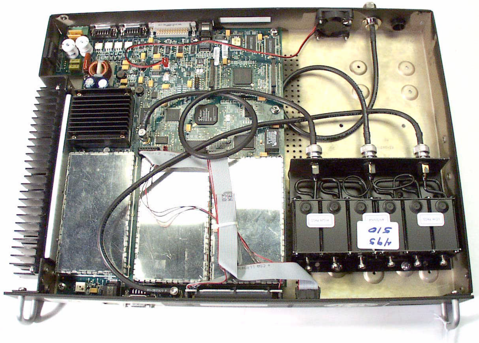
EXHIBIT 12 INTERNAL EUT PHOTOS FCC ID: E5M-LEDR400S
