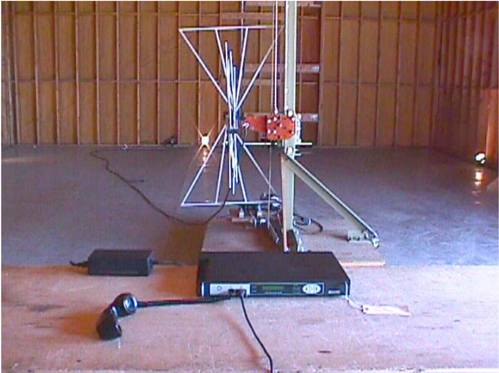
EXHIBIT 10 TEST SETUP PHOTOS RADIATED EMISSIONS AT 3 METERS DISTANCE FCC ID: E5M-LEDR400S
