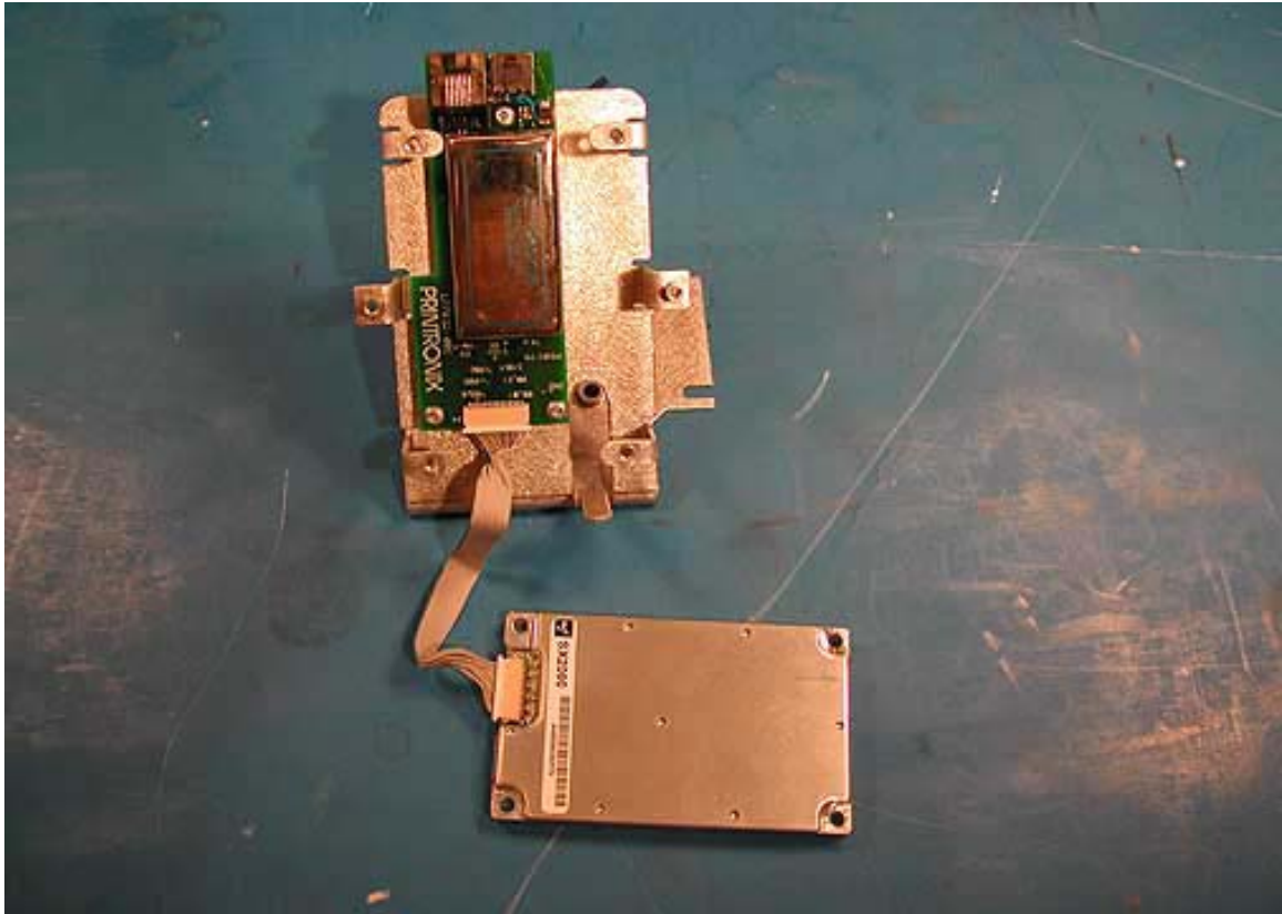
Card Bracket 4
