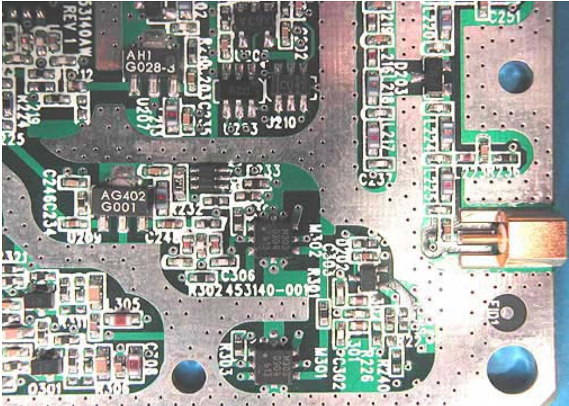
TX PCB 6
