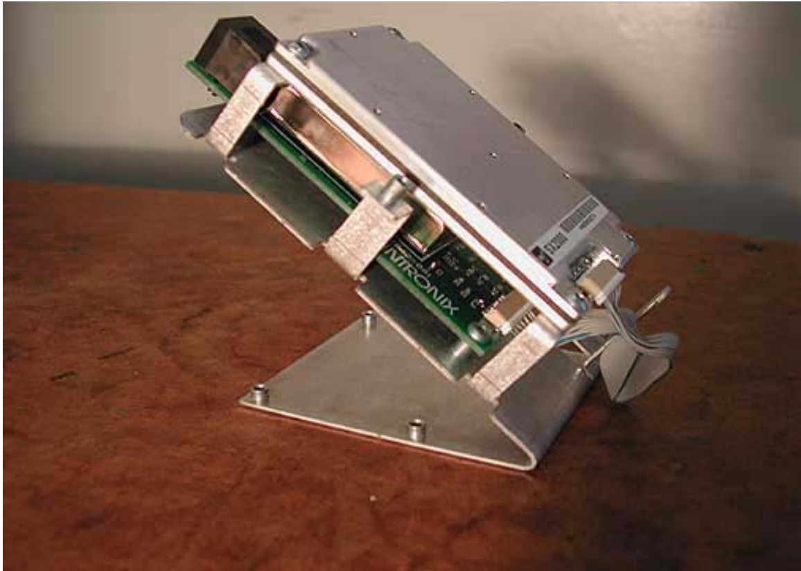
Card Bracket 3
