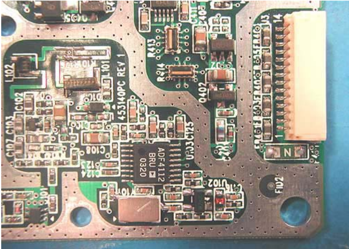
TX PCB 3
