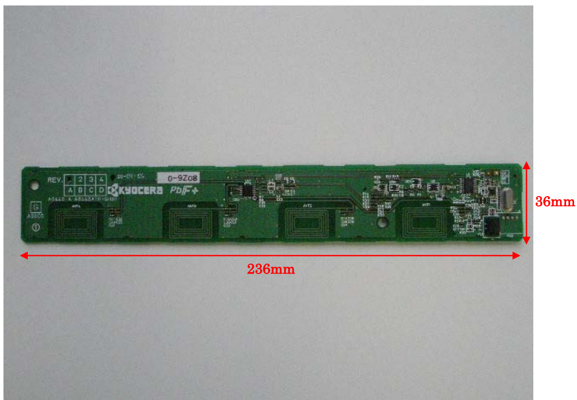
Picture of RFID-P.W.B.(A0440)
