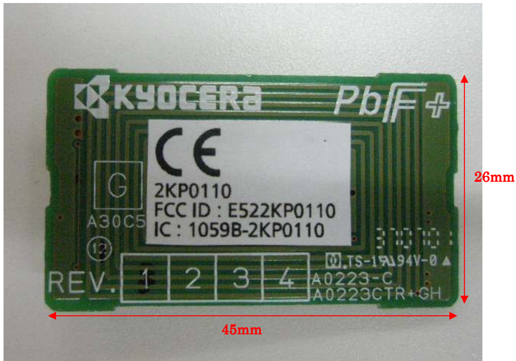
Picture of RFID-P.W.B.(2KP0110)
