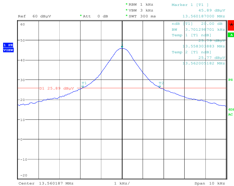
Figure 4: 20dB Bandwidth
