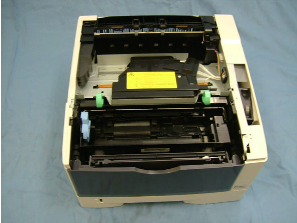
Top view with top cover removed
