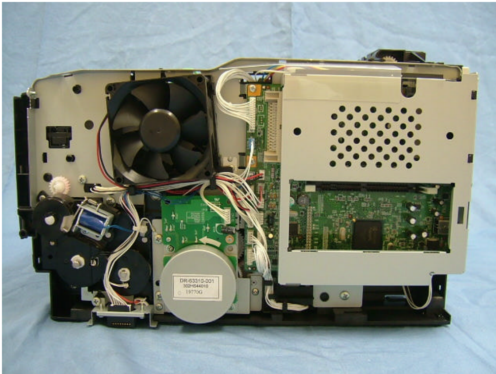
Right side view with right cover removed
