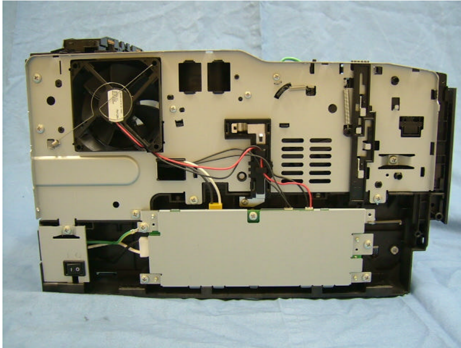
Left side view with left cover removed
