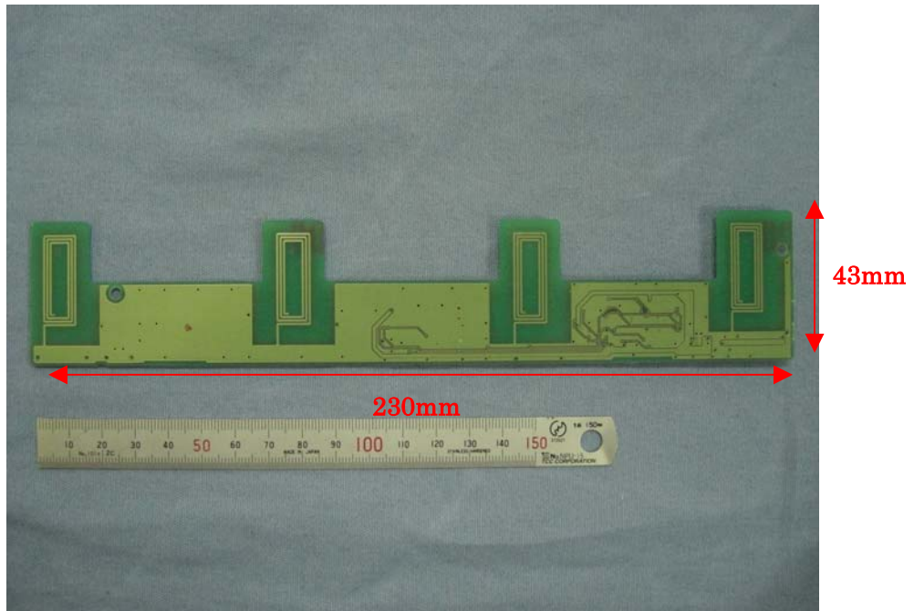
Picture of RFID-P.W.B.
