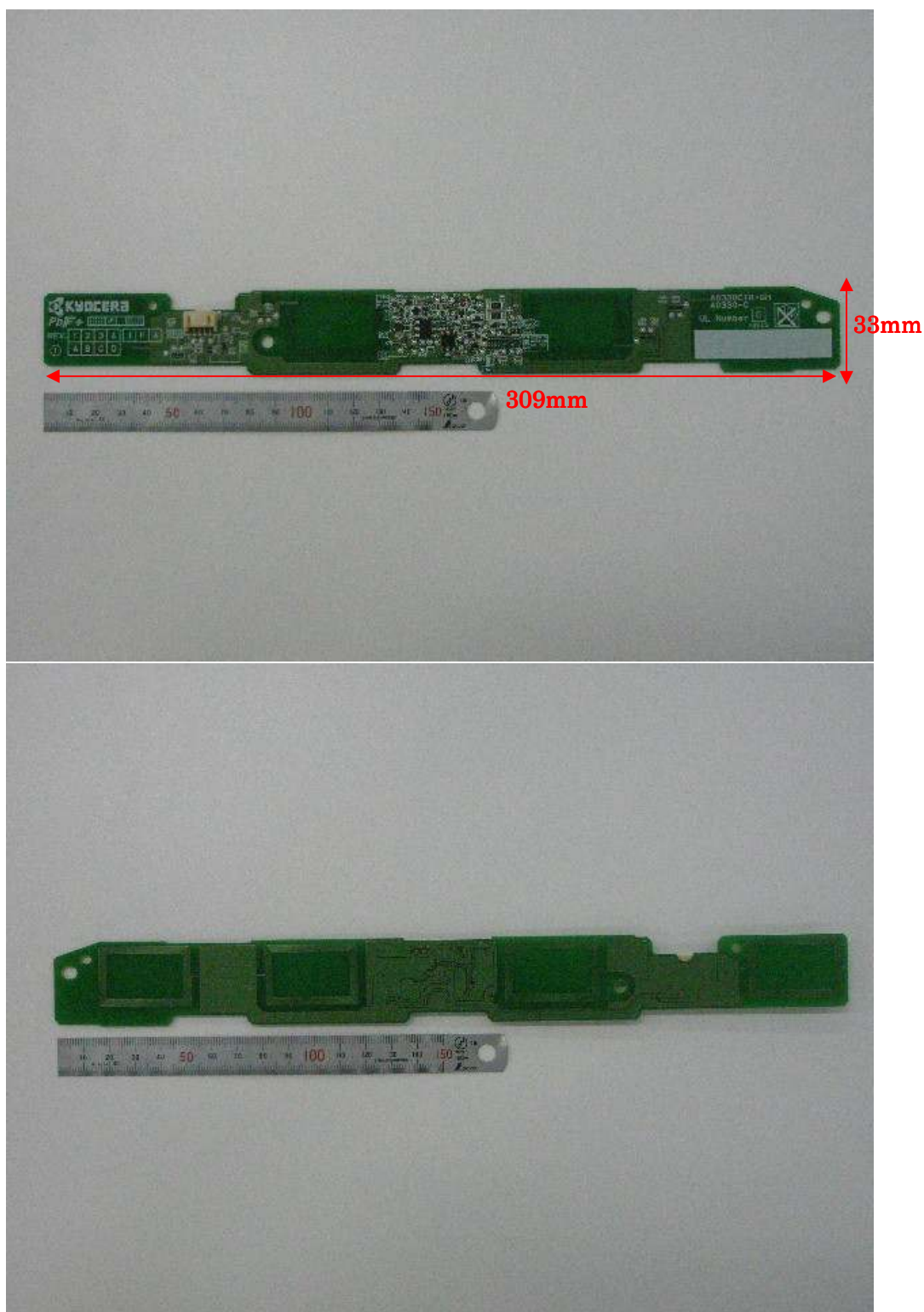
Picture of RFID-P.W.B.(A0330)
